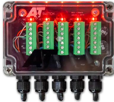
Ethernet Switch
