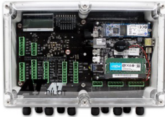
Pilot Processor
